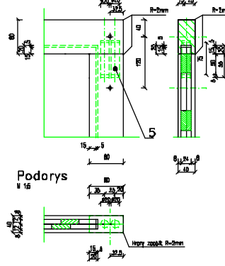
Detail X M 15
