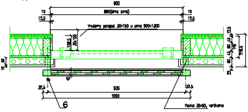
REZ B-B M 110
